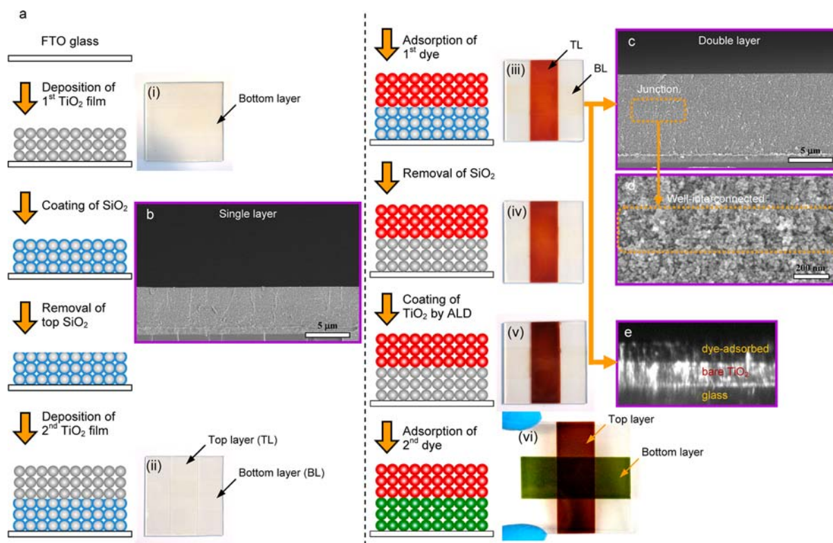
Figure 2. (a) Schematic procedure for the fabrication of two-color-photoanodes. (b, c) Scanning electron microscope (SEM) images of single and double layered, nanoporous TiO 2 films as indicated. (d) Magnified SEM image at the junction area between top and bottom TiO 2 layers. (e) Cross-sectional optical microscope image after the first chromophore adsorbed. (i)–(vi), Photographs of TiO 2 films at each step.
