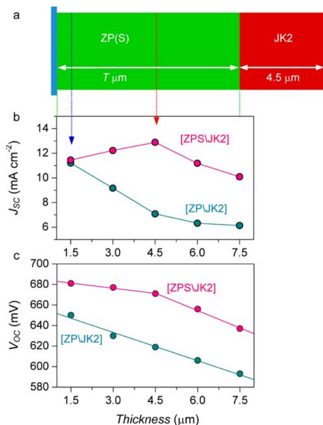
Figure 5. Correlation between electron collection length and actual film thickness of lower layer. (a) Schematic illustration for the configuration of [ZP\JK2] or [ZPS\JK2], and (b) plot of short-circuit current and (c) open-circuit voltage changes versus lower-layer thickness.
