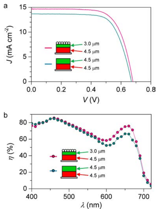
Figure 6. JV (a) and IPCE (b) curves of [JK2\ZPS] with and without scattering layer as indicated.
