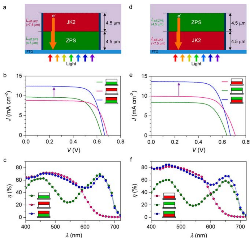
Figure 4. (a) and (d) Schematic illustration for the configuration and electron collection of a two-color photoanode with JK2 and ZPS. (b) JV curves and (c) IPCE spectra of [ZPS\JK2], [-\JK2], and [ZPS\JK2] as indicated. (e) JV curves and (f) IPCE spectra of [JK2\ZPS], [-\ZPS], and [JK2\ZPS] as indicated.
