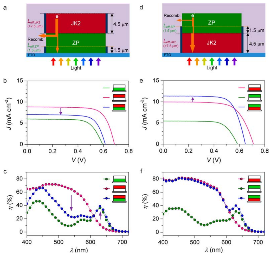
Figure 3. (a) and (d) Schematic illustration for the configuration and electron collection of a two-color photoanode with JK2 and ZP chromophores. (b) JV curves and (c) IPCE spectra of [ZP\JK2], [-\JK2], and [ZP] as indicated. (e) JV curves and (f) IPCE spectra of [JK2\ZP], [-\ZP], and [JK2] as indicated.
